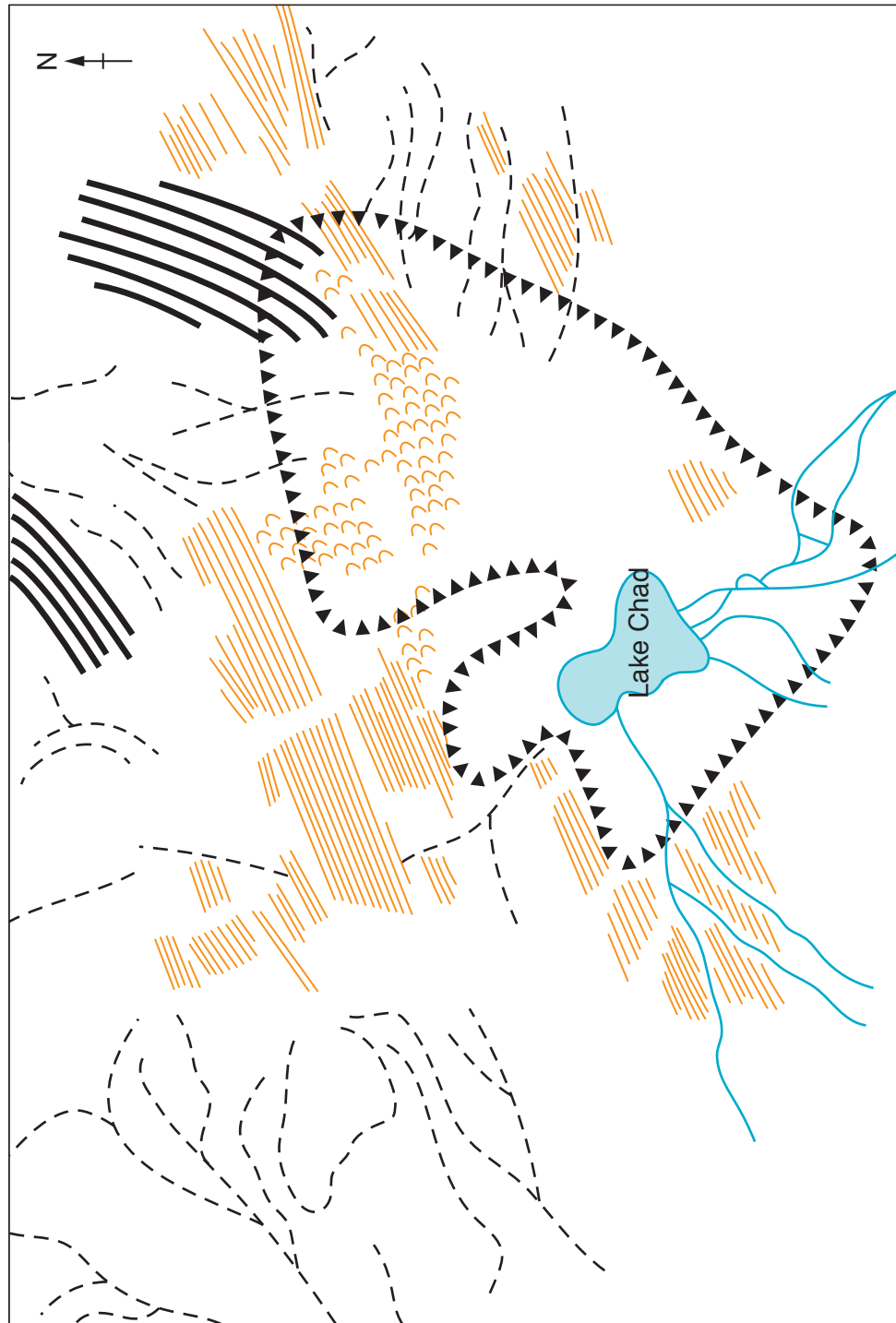
Landforms found in part of the southern Sahara Desert
